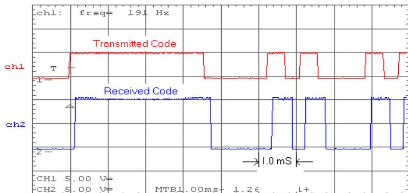
PM3370A Typical I/R Code Transmission RTX/RRX-11
