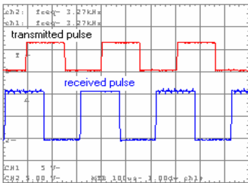
PM3370A 150 \mu Sec Pulse Transmission
